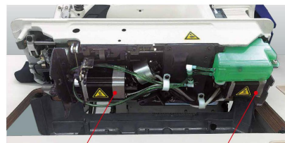
Motor for vertically-driven digital feed mechanism
